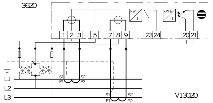
K420iJps and K410iJps
